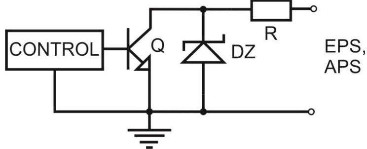
Fig. 4. Electrical diagram of OC outputs.
